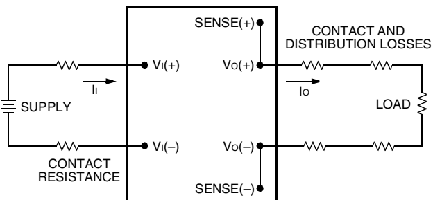
Figure 18. Peak-to-Peak Output Noise Measurement Test Setup
