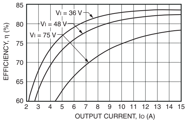
Figure 5. Typical QHW075Y1 Converter Efficiency vs. Output Current at Room Temperature
