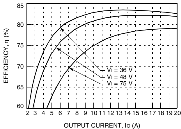
Figure 6. Typical QHW100Y1 Converter Efficiency vs. Output Current at Room Temperature
