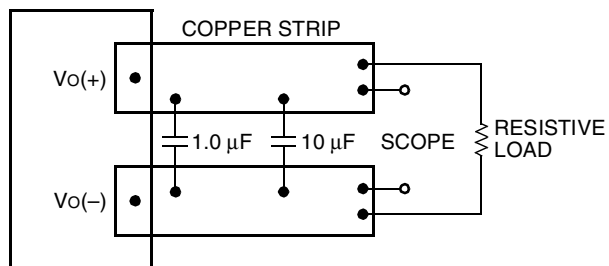
Figure 17. Input Reflected-Ripple Test Setup
