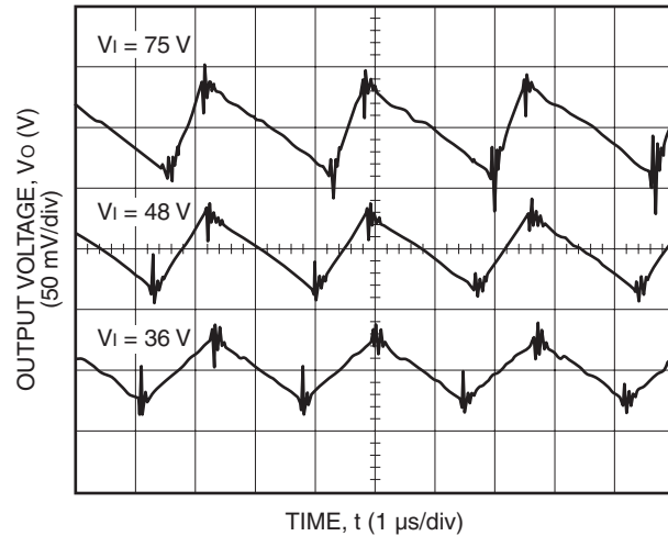
Figure 7. Typical QHW050Y1, Output Ripple Voltage at Room Temperature; I_o = I_{o, max}
