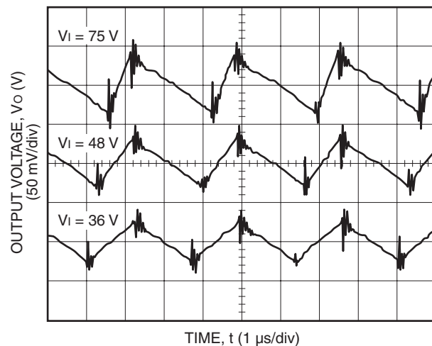
Figure 8. Typical QHW075Y1, Output Ripple Voltage at Room Temperature; I_o = I_{o, max}
